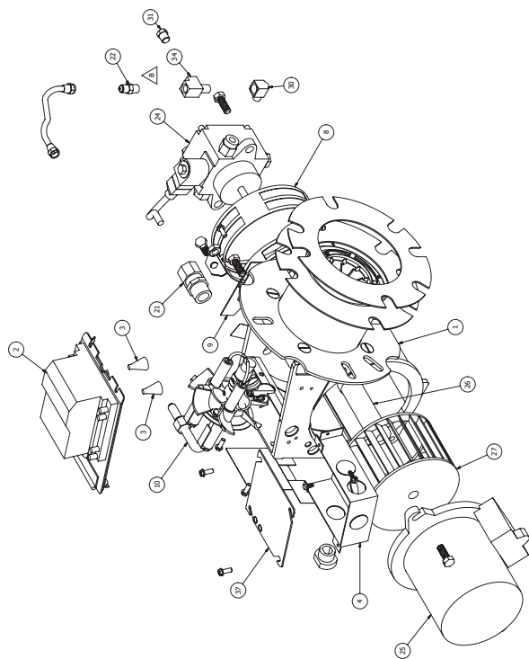
EXPLODED VIEW
